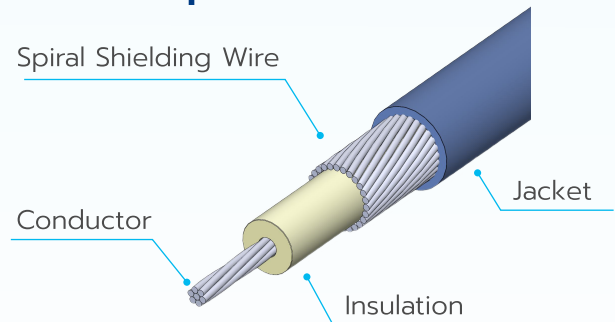
MCX Cable Structure
