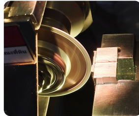
Profile grinding
